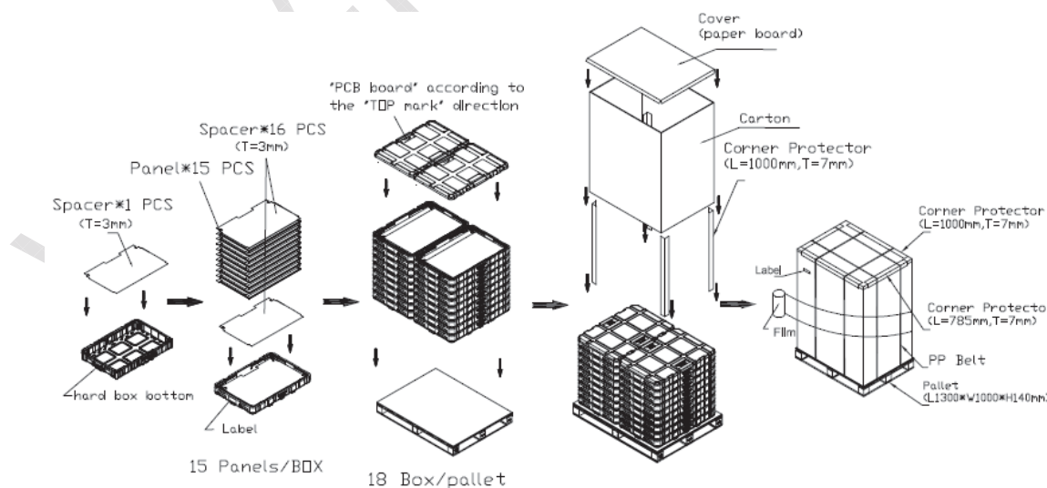
Figure.9-2 packaging method (CELL 2)
